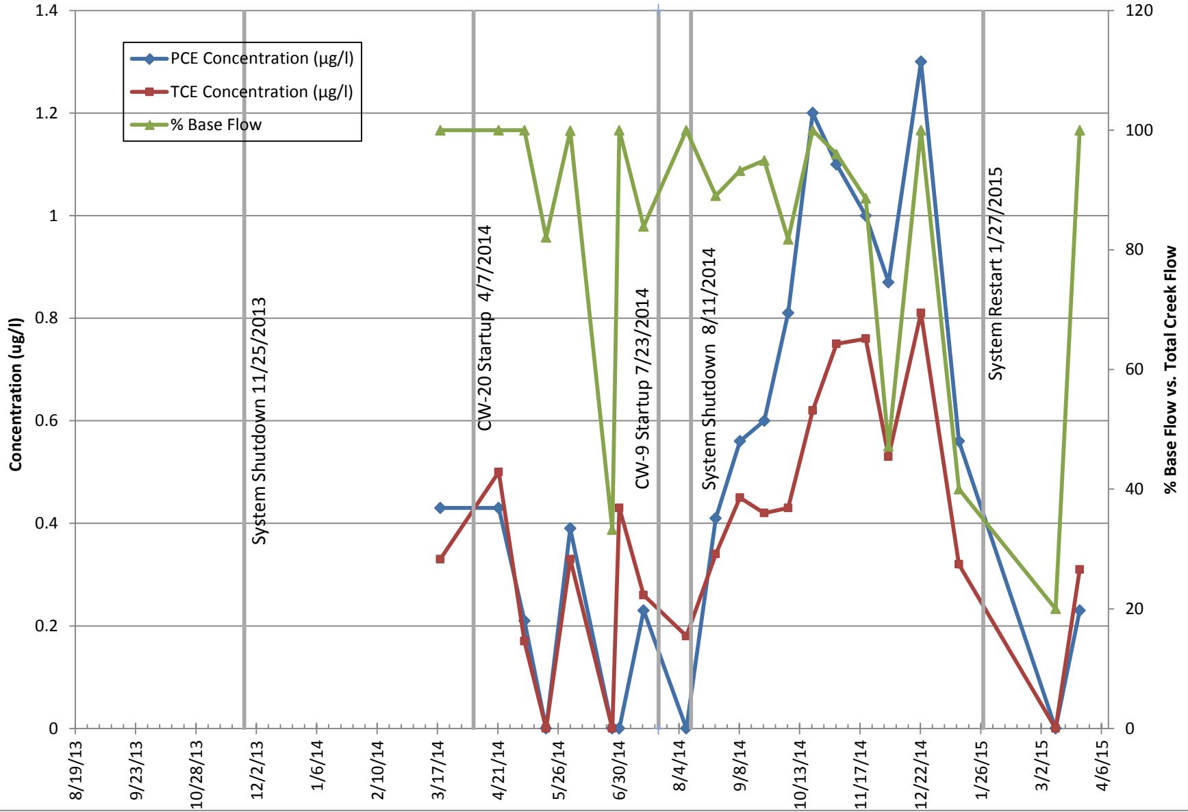
FIGURE 3.5-21 SW-29 Concentration vs Time compared to % Baseflow
